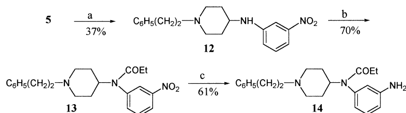
Scheme 2. (a) 3\text{-Nitroaniline/NaBH}_3\text{CN/MeOH/3 \AA sieves} ; (b) (\text{EtCO})_2\text{O} ; (c) \text{H}_2/\text{Pd/C/AcOH/35-40 psi} .
