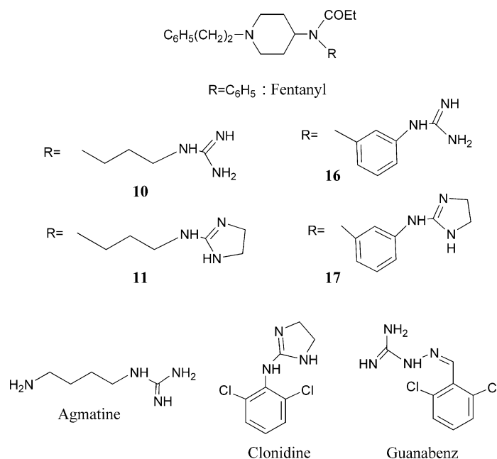
Figure 1. Chemical structure of fentanyl, compounds tested biologically included in this work and some known imidazoline ligands.
