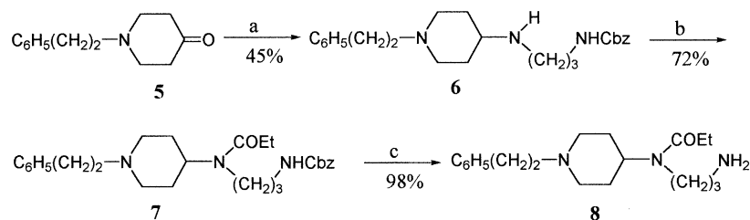
Scheme 1. (a) 4/\text{NaBH}_3\text{CN/MeOH/3 \AA sieves} ; (b) (\text{EtCO})_2\text{O} ; (c) \text{H}_2/\text{Pd/C/AcOH/35-40 psi} .
