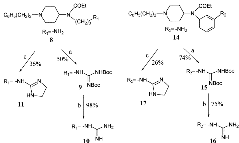
Scheme 3. (a) (\text{BocNH})_2\text{CS/TEA/HgCl}_2/\text{CH}_2\text{Cl}_2/0^\circ\text{C} ; (b) \text{TFA/CH}_2\text{Cl}_2 ; (c) 2-methylthioimidazolinium iodide/MeOH.
